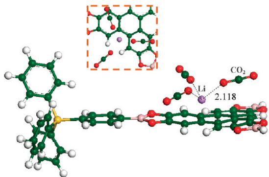
(b) Adsorption of three CO 2 molecules on Li-doped COFs with B.E. = -20.140 kcal/mol
