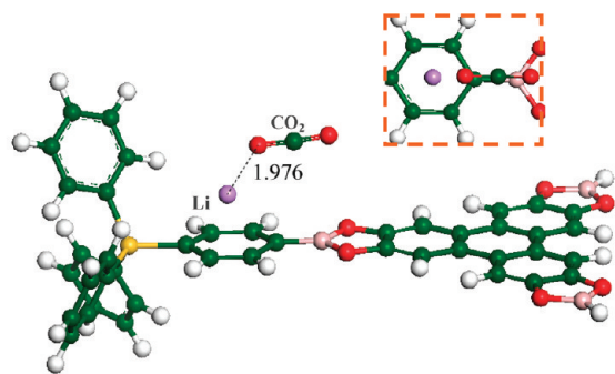
(a) Adsorption of a single CO 2 molecule on Li-doped COFs with B.E. = -10.074 kcal/mol
