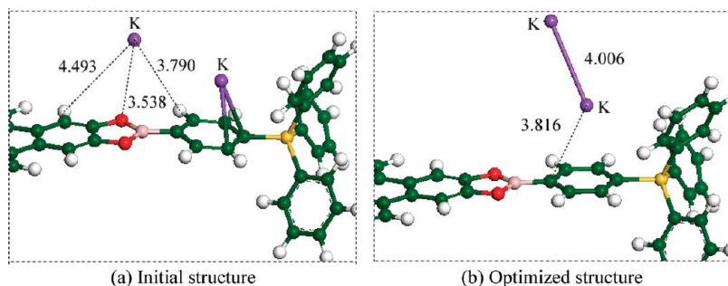
Figure 7. Adsorption geometries of two K atoms in COFs: (a) initial structure and (b) optimized structure. The binding energy of two K atoms in COFs is -18.414 kcal/mol. The measured distances from the adsorbed K atoms to the surface are presented in Å. C, O, B, H, Si, and K atoms are shown as green, red, pink, white, yellow, and purple colors, respectively.
