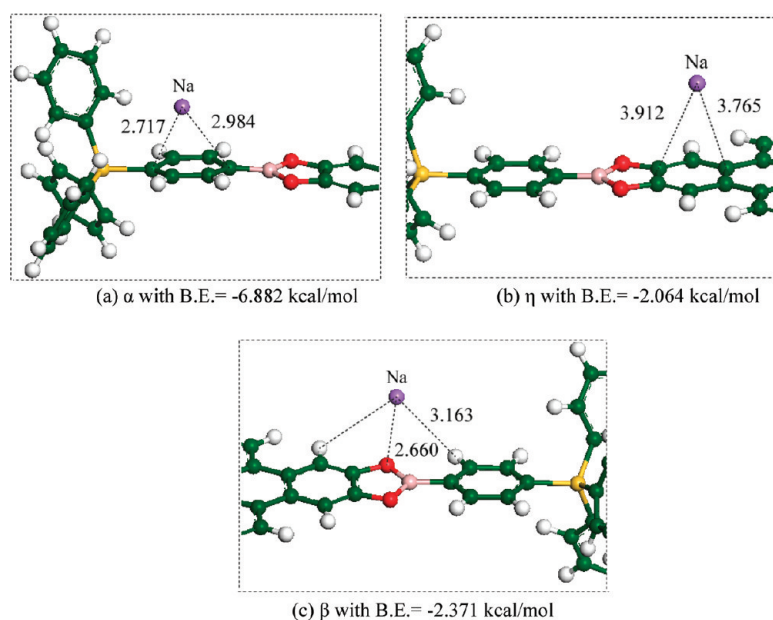
Figure 4. Optimized adsorption sites of Na in the 3D COFs: (a) \alpha , (b) \eta , and (c) \beta . The calculated binding energies are also shown correspondingly. The measured distances from the adsorbed Na atom to the surface are presented in Å. C, O, B, H, Si, and Na atoms are shown as green, red, pink, white, yellow, and purple colors, respectively.
